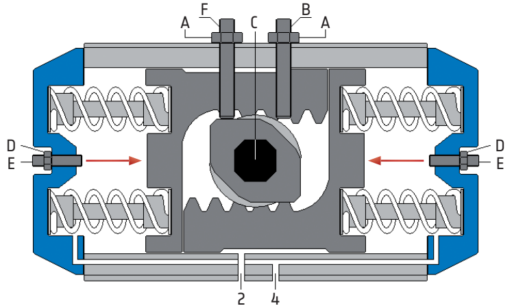
Basic position 0°
