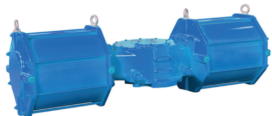
Scotch-Yoke version / 90°
